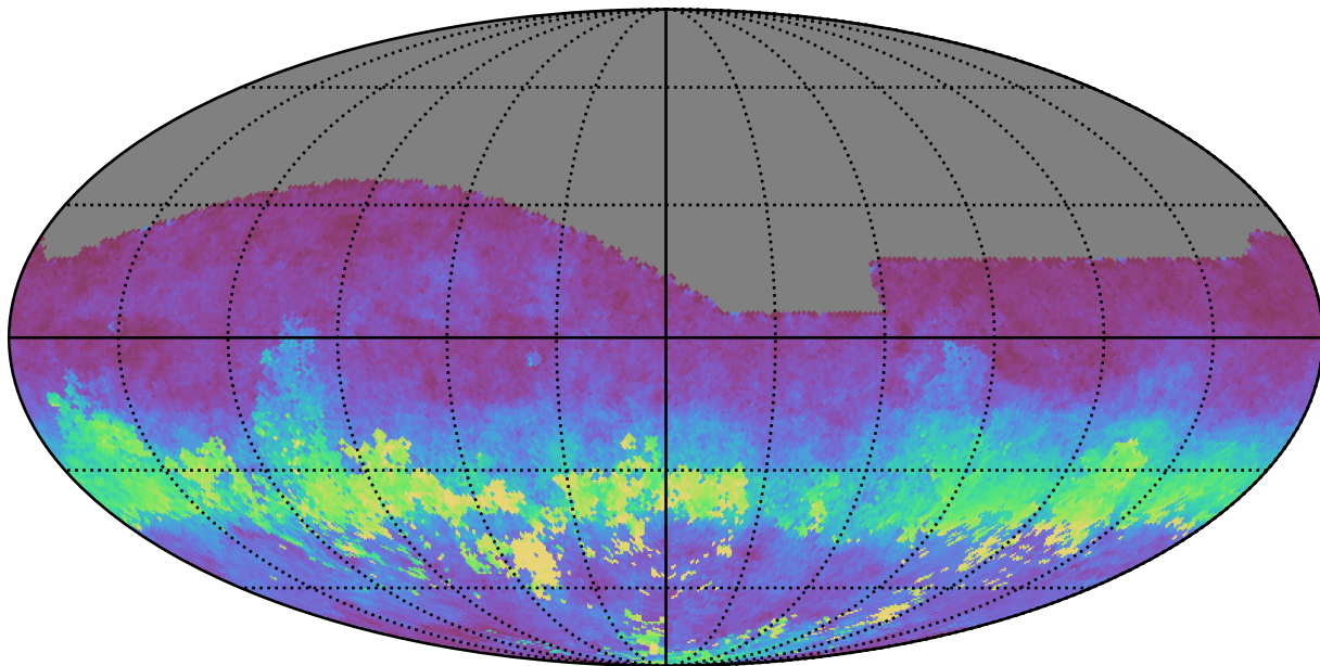
baseline_v3.5_10yrs All sky g band: AngleRms rotSkyPos
