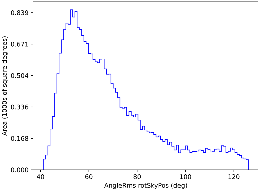
baseline_v3.5_10yrs All sky g band: AngleRms rotSkyPos
