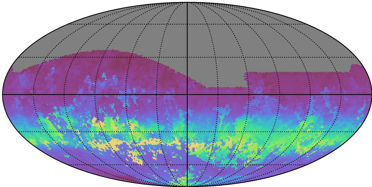
baseline_v3.5_10yrs All sky all bands: AngleRms rotSkyPos
