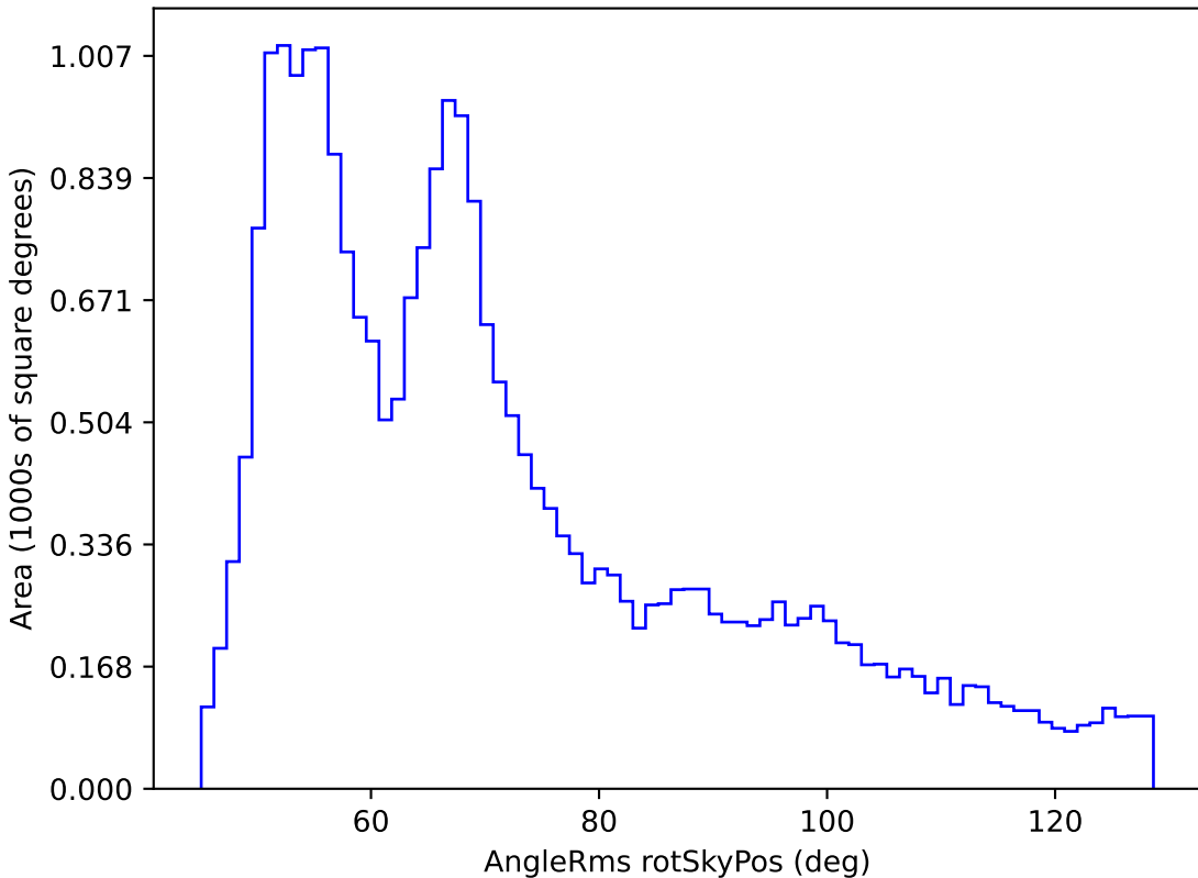
baseline_v3.5_10yrs All sky all bands: AngleRms rotSkyPos
