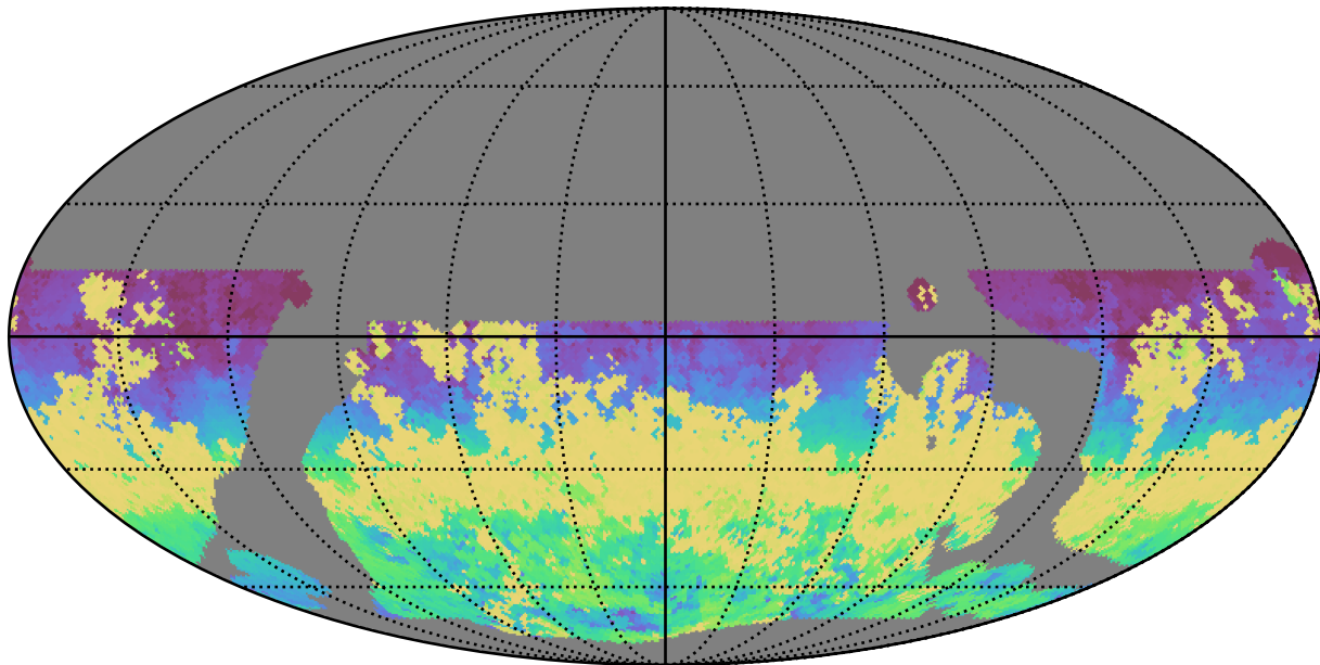
baseline_v3.5_10yrs WFD z band: AngleRange rotSkyPos
