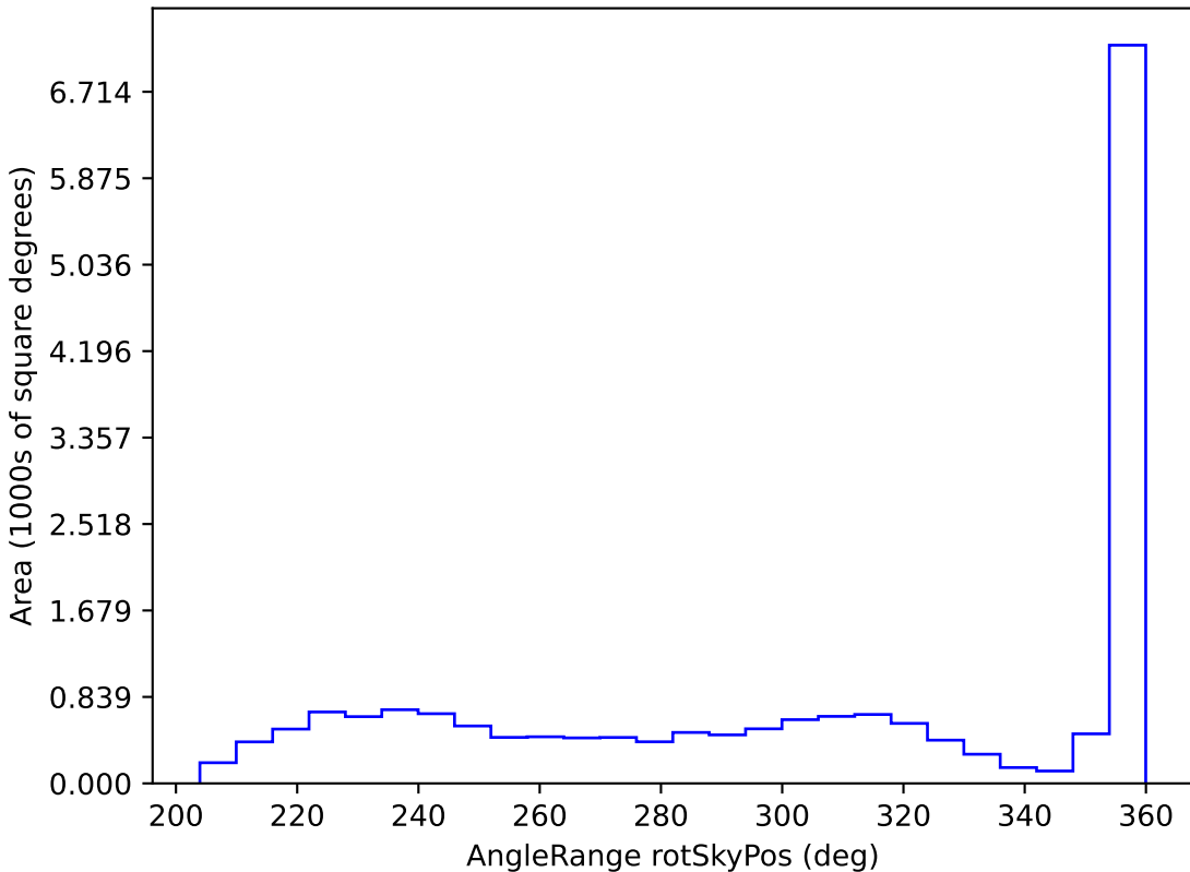
baseline_v3.5_10yrs WFD z band: AngleRange rotSkyPos
