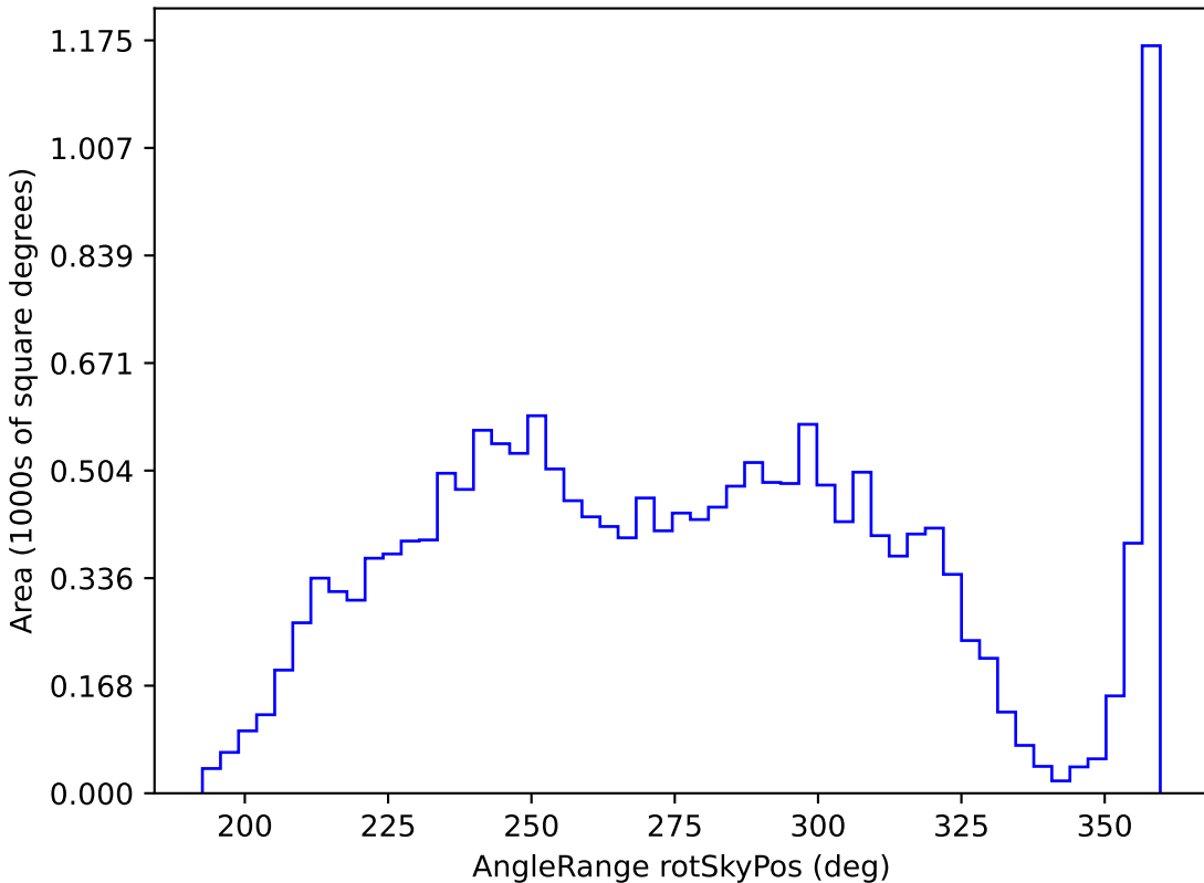
baseline_v3.5_10yrs WFD y band: AngleRange rotSkyPos
