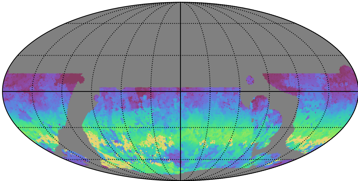
baseline_v3.5_10yrs WFD u band: AngleRange rotSkyPos
