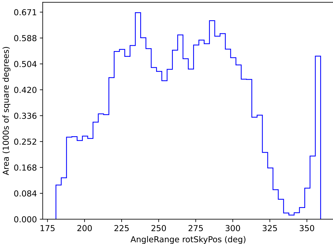
baseline_v3.5_10yrs WFD u band: AngleRange rotSkyPos
