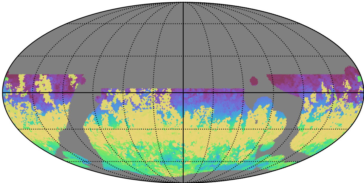
baseline_v3.5_10yrs WFD r band: AngleRange rotSkyPos
