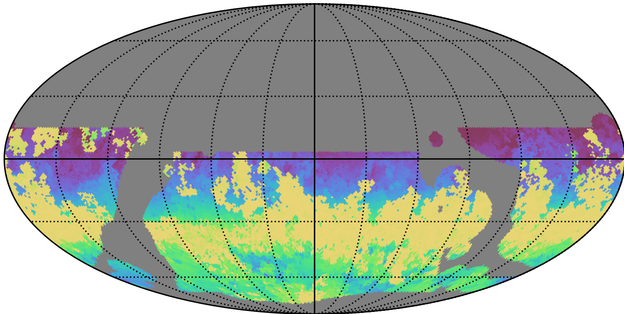
baseline_v3.5_10yrs WFD i band: AngleRange rotSkyPos
