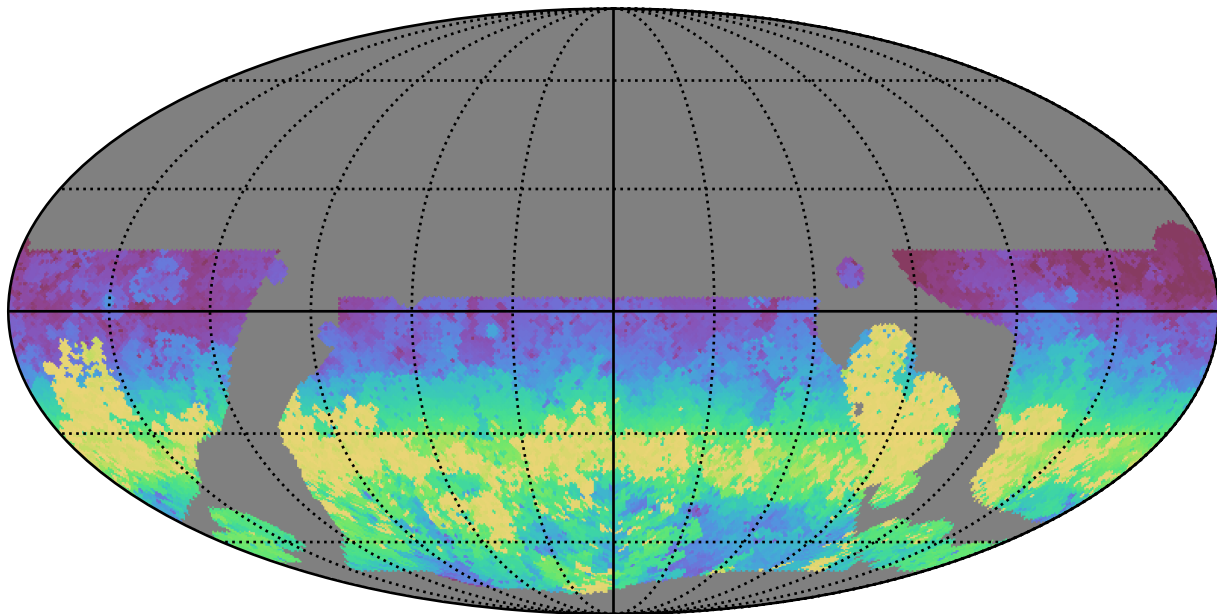
baseline_v3.5_10yrs WFD g band: AngleRange rotSkyPos
