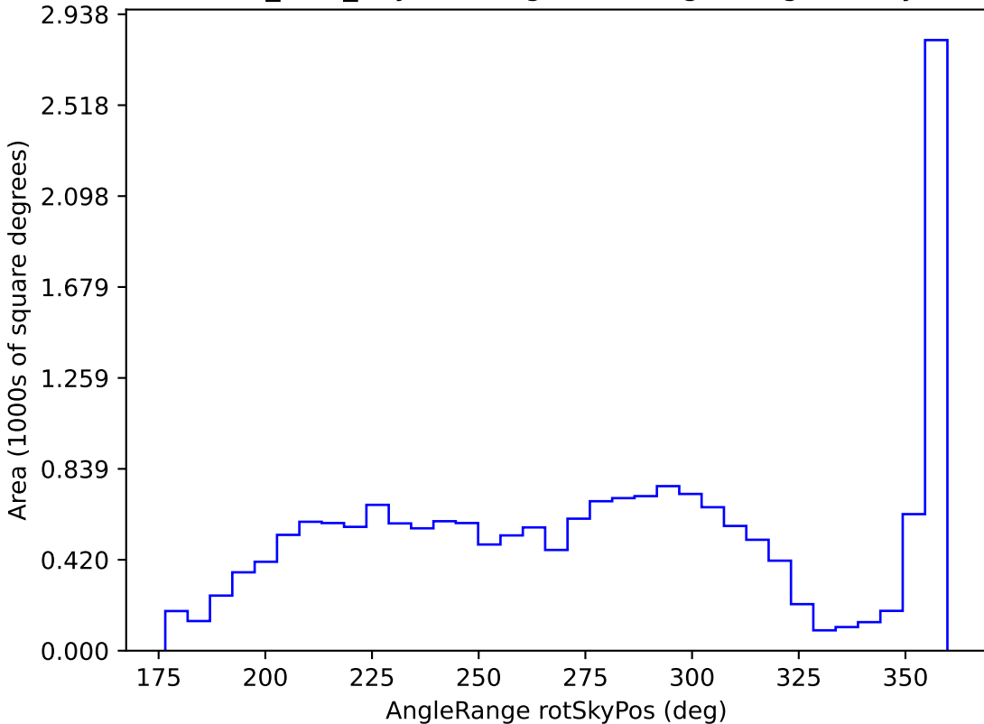
baseline_v3.5_10yrs WFD g band: AngleRange rotSkyPos
