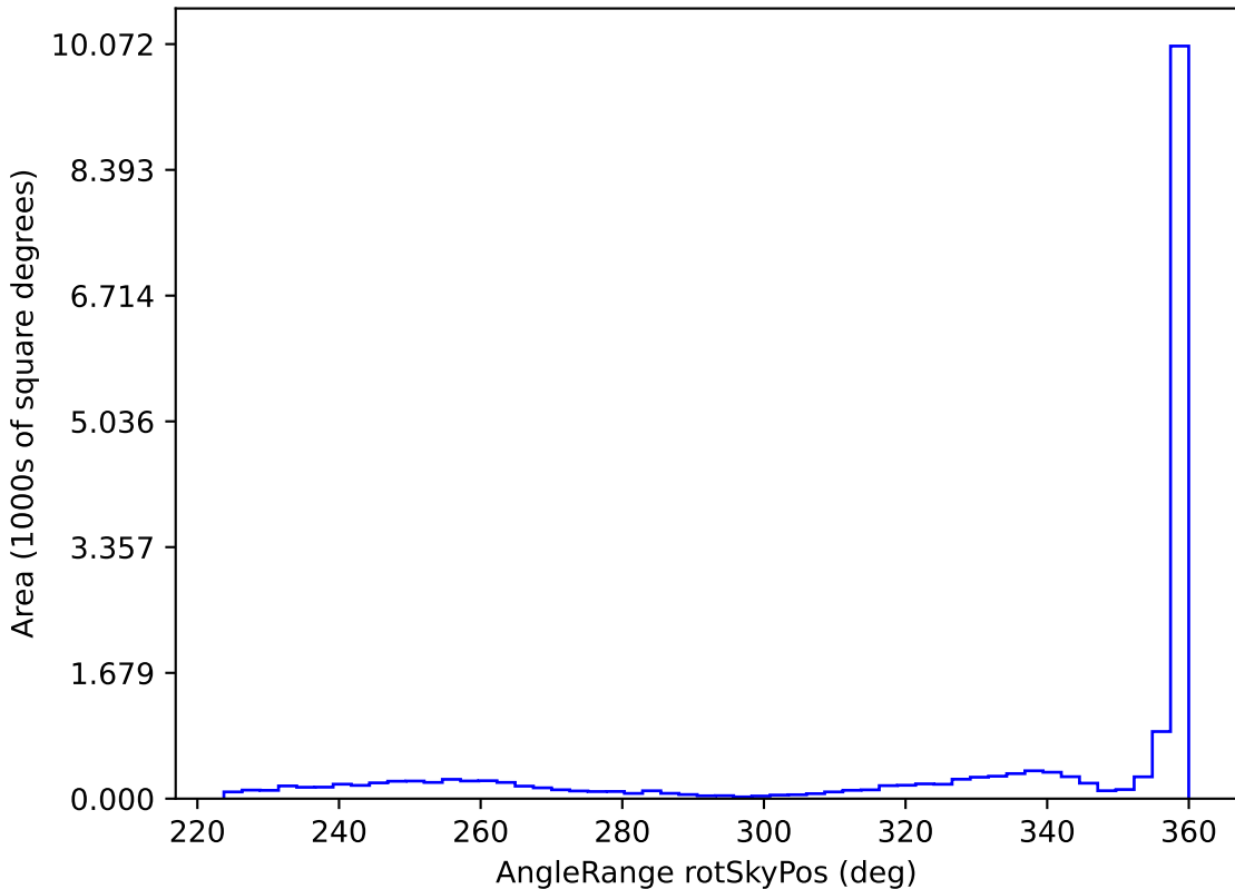
baseline_v3.5_10yrs WFD all bands: AngleRange rotSkyPos
