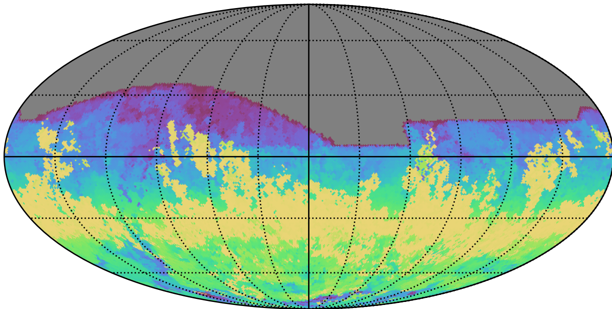
baseline_v3.5_10yrs All sky z band: AngleRange rotSkyPos
