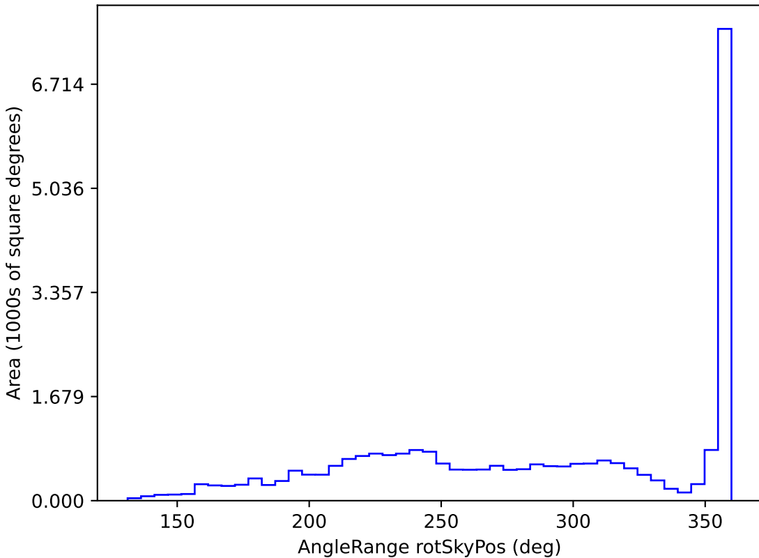
baseline_v3.5_10yrs All sky z band: AngleRange rotSkyPos
