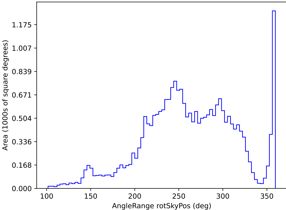
baseline_v3.5_10yrs All sky y band: AngleRange rotSkyPos
