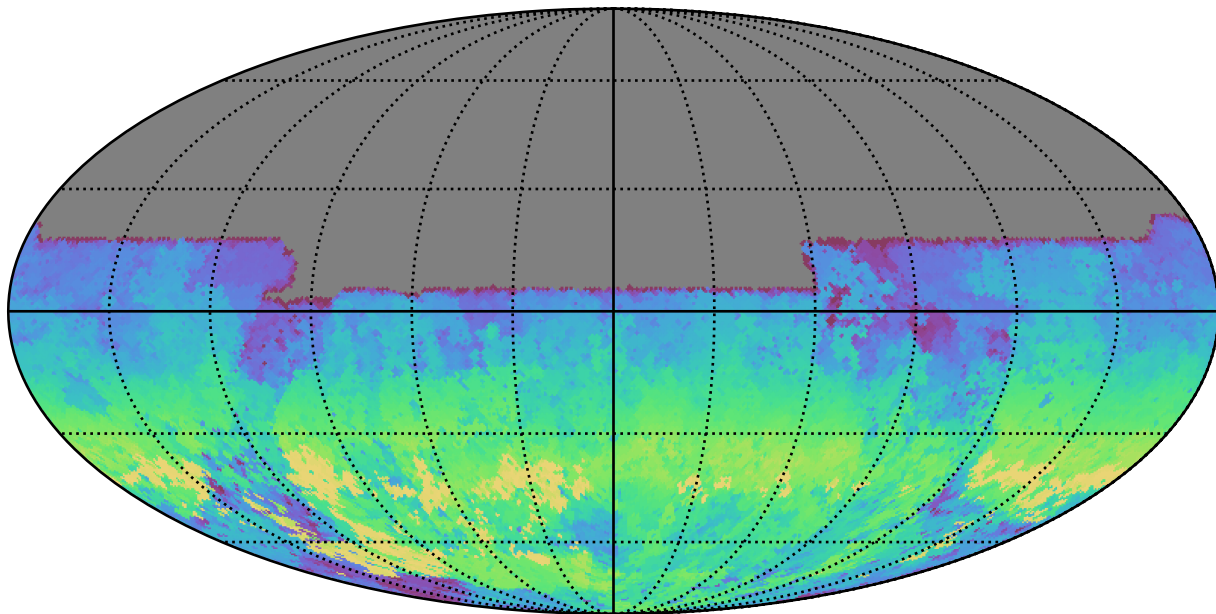
baseline_v3.5_10yrs All sky u band: AngleRange rotSkyPos
