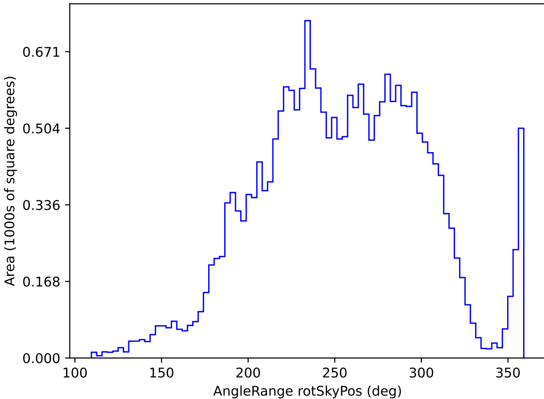
baseline_v3.5_10yrs All sky u band: AngleRange rotSkyPos
