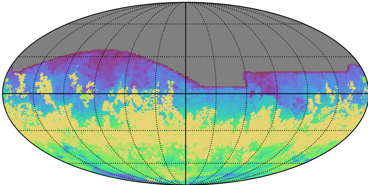
baseline_v3.5_10yrs All sky r band: AngleRange rotSkyPos
