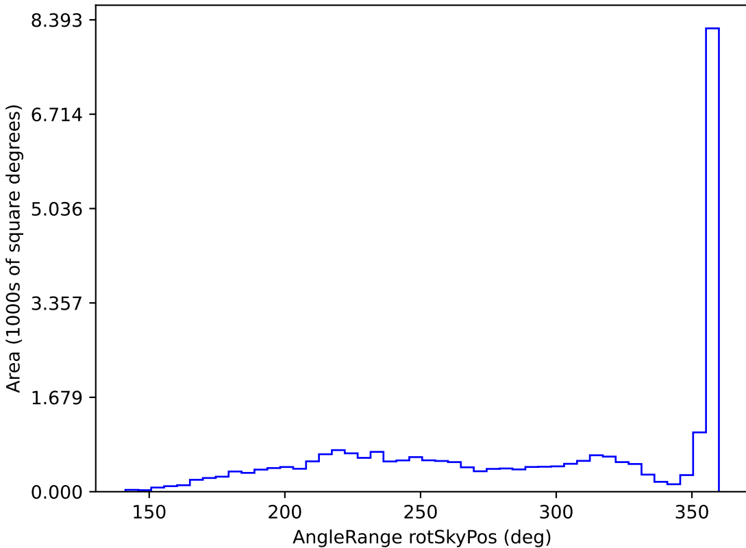
baseline_v3.5_10yrs All sky r band: AngleRange rotSkyPos
