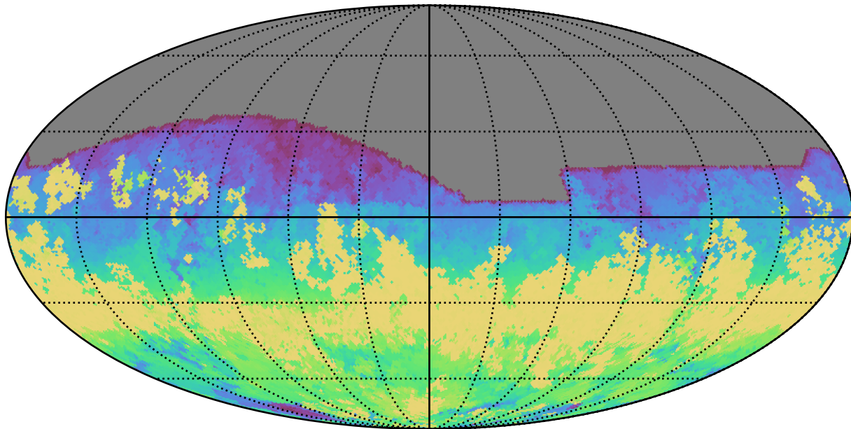
baseline_v3.5_10yrs All sky i band: AngleRange rotSkyPos
