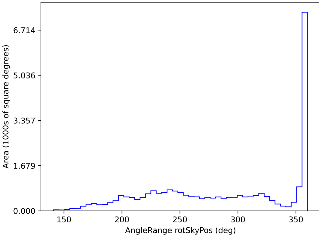
baseline_v3.5_10yrs All sky i band: AngleRange rotSkyPos
