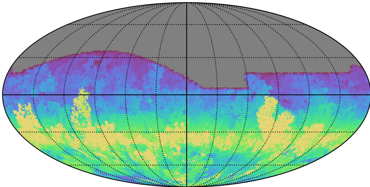
baseline_v3.5_10yrs All sky g band: AngleRange rotSkyPos
