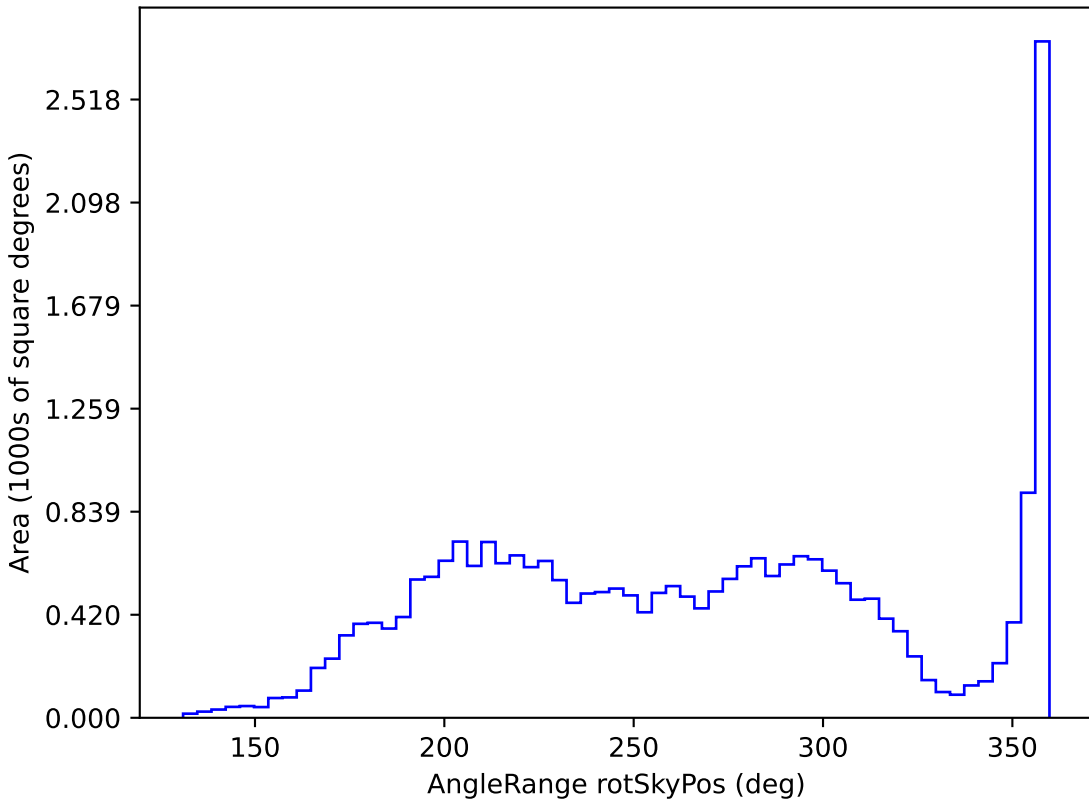
baseline_v3.5_10yrs All sky g band: AngleRange rotSkyPos
