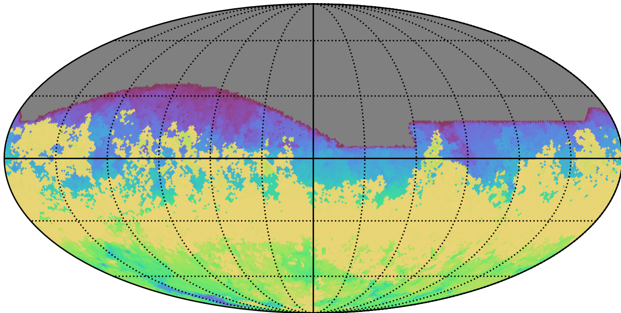
baseline_v3.5_10yrs All sky all bands: AngleRange rotSkyPos
