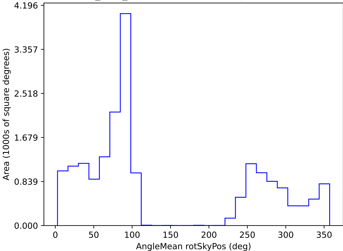
baseline_v3.5_10yrs WFD z band: AngleMean rotSkyPos
