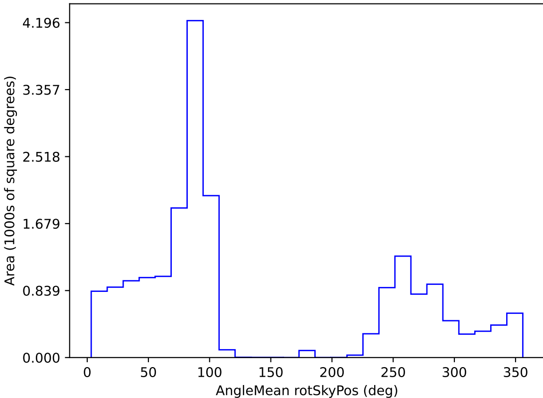
baseline_v3.5_10yrs WFD r band: AngleMean rotSkyPos
