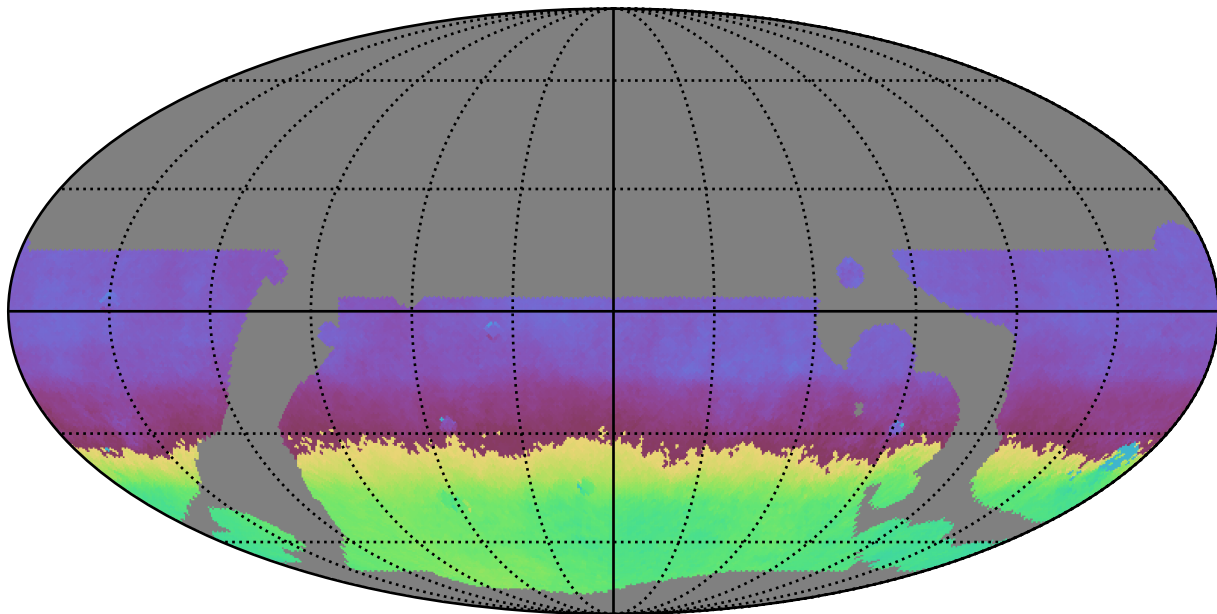
baseline_v3.5_10yrs WFD i band: AngleMean rotSkyPos
