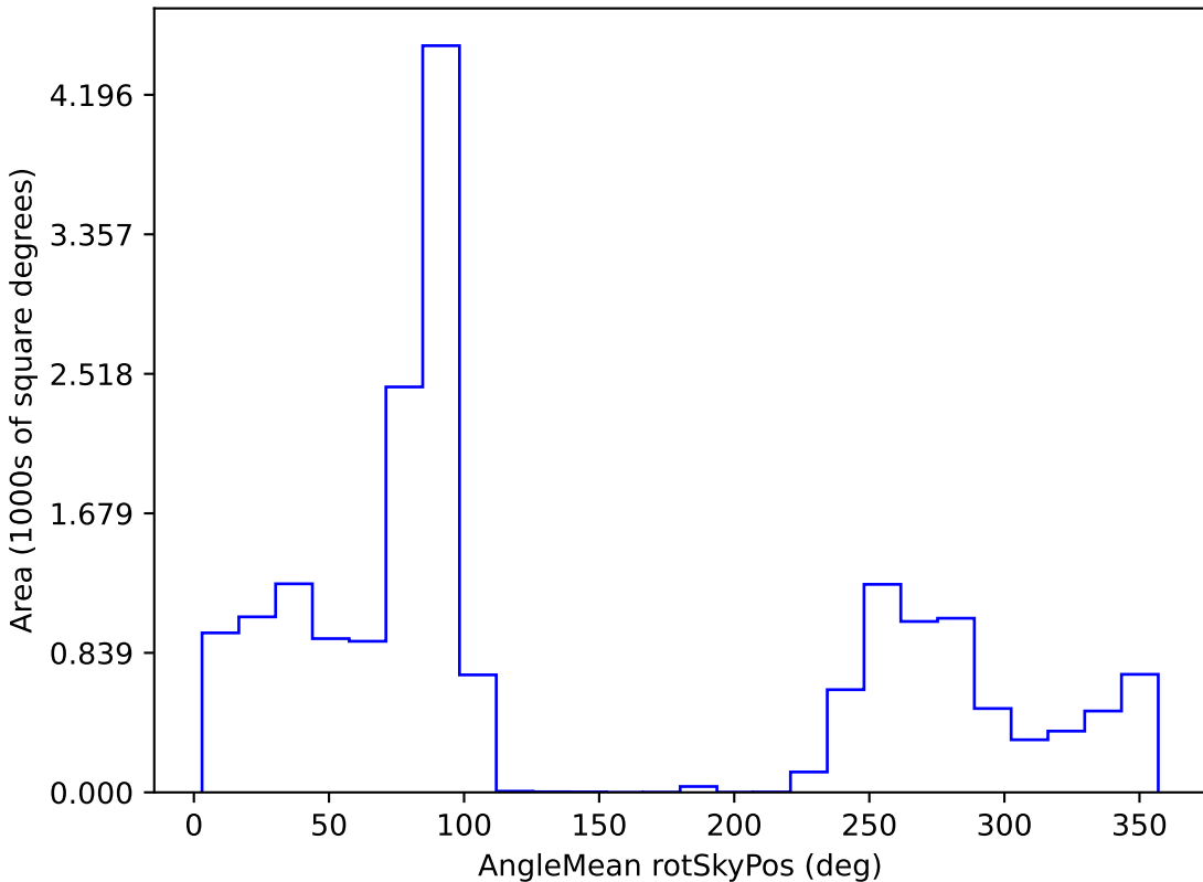
baseline_v3.5_10yrs WFD i band: AngleMean rotSkyPos
