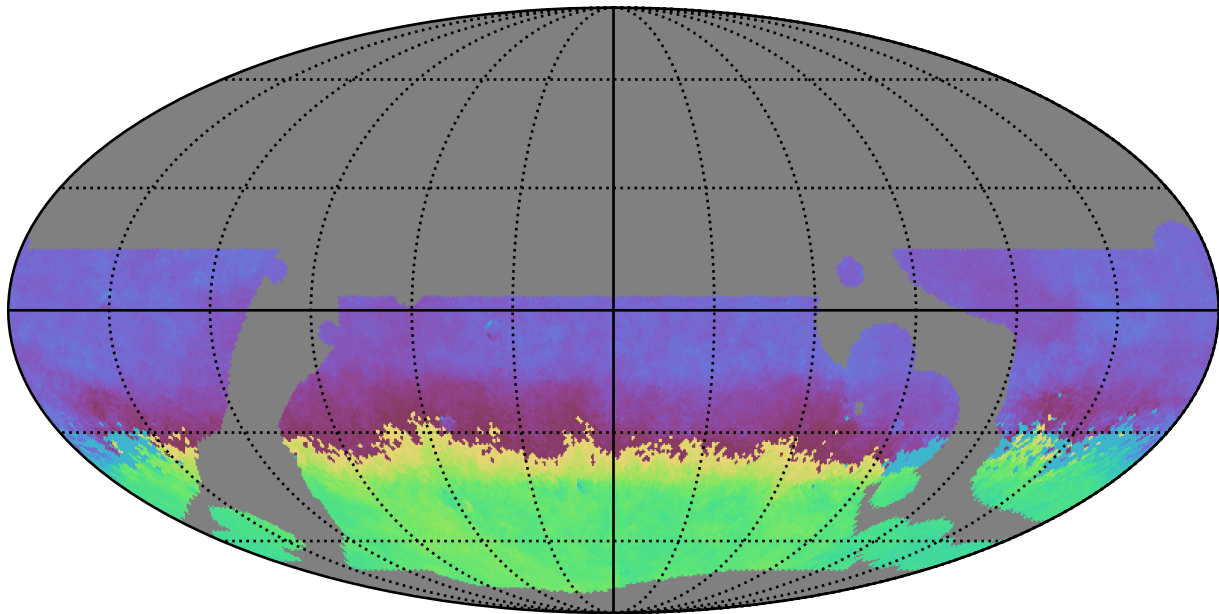
baseline_v3.5_10yrs WFD g band: AngleMean rotSkyPos
