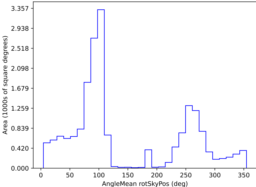
baseline_v3.5_10yrs WFD g band: AngleMean rotSkyPos
