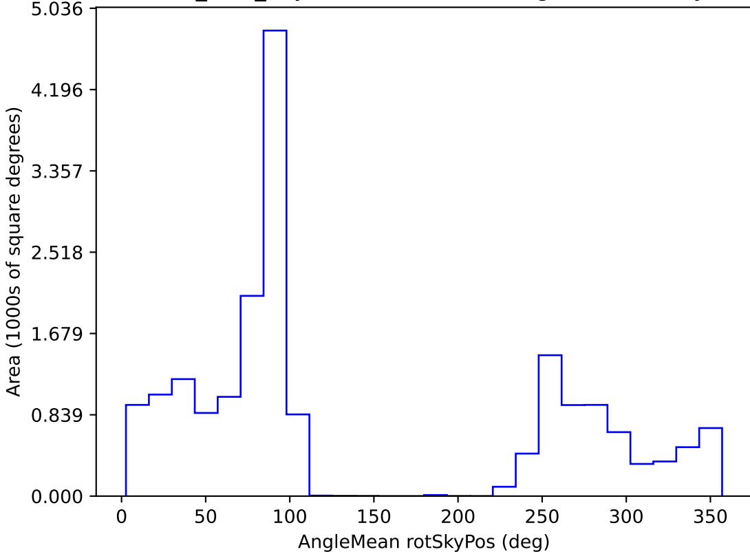
baseline_v3.5_10yrs WFD all bands: AngleMean rotSkyPos
