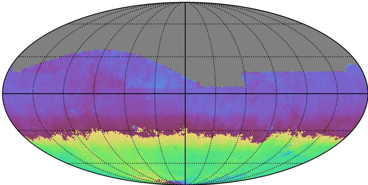
baseline_v3.5_10yrs All sky z band: AngleMean rotSkyPos
