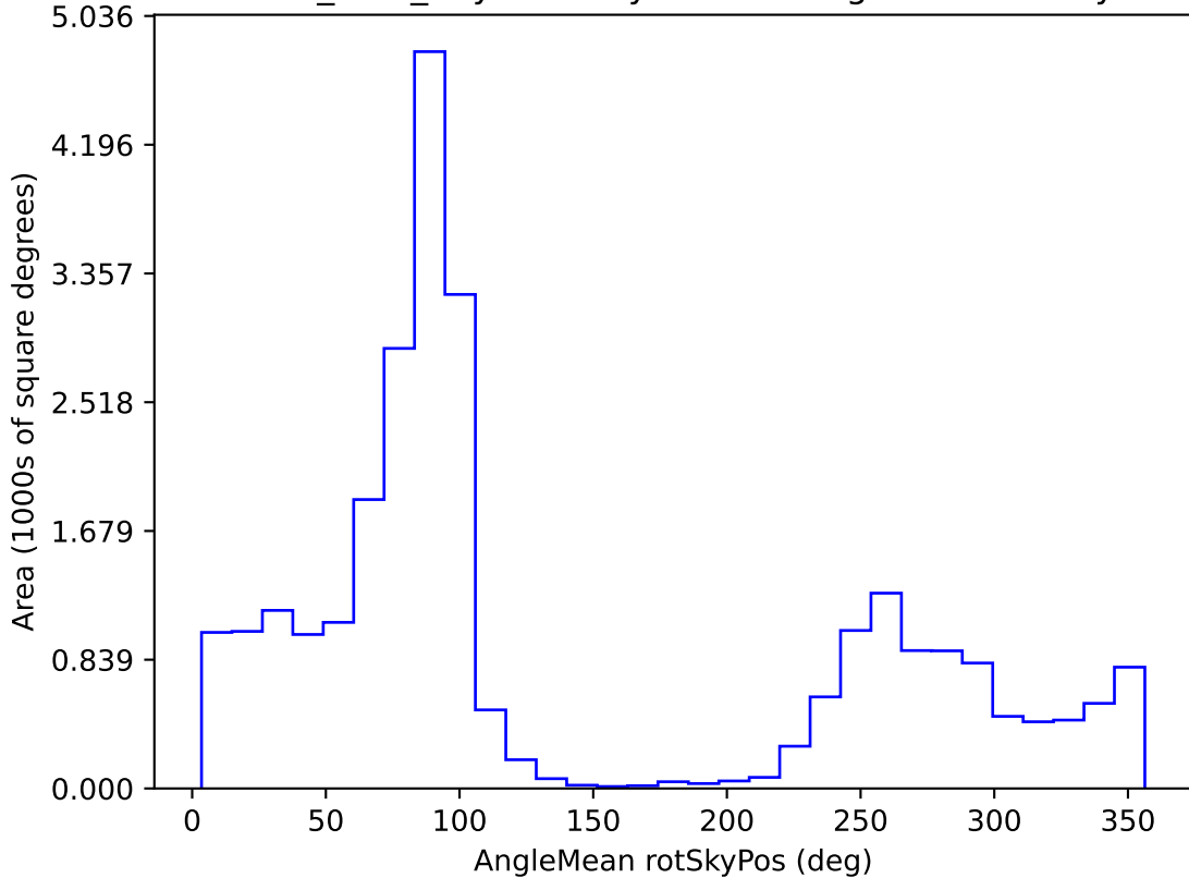
baseline_v3.5_10yrs All sky z band: AngleMean rotSkyPos
