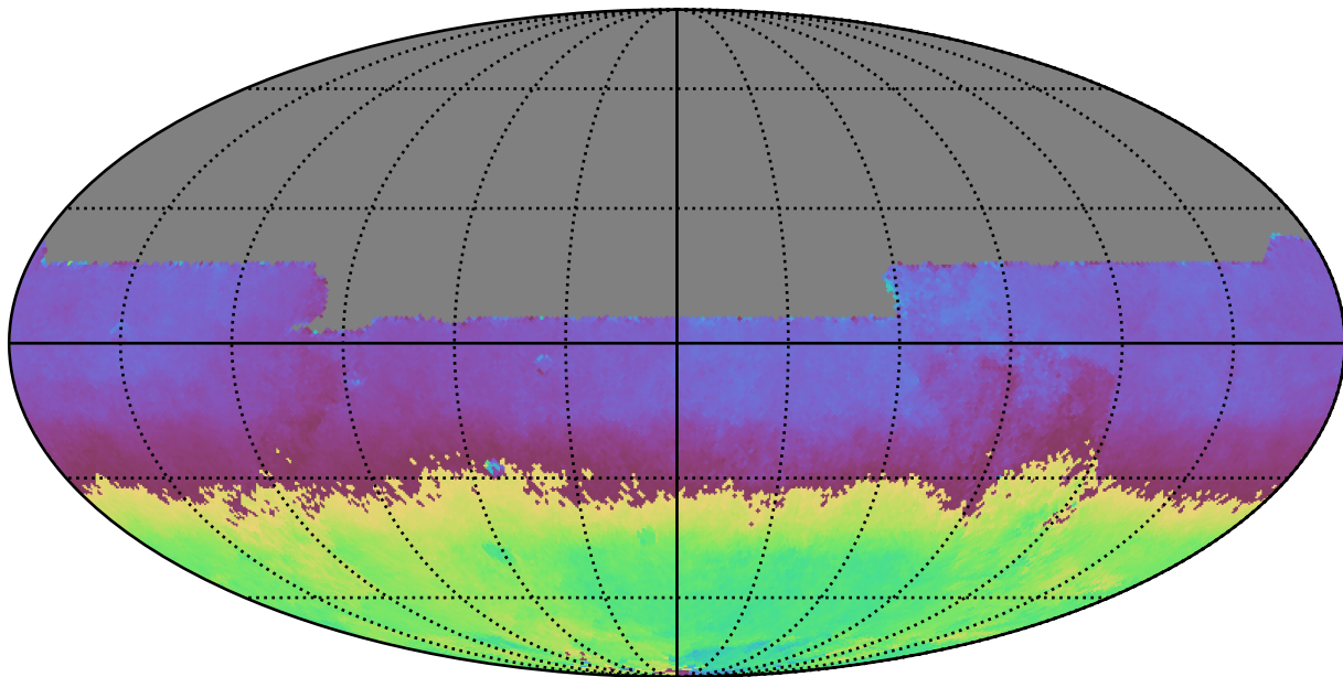
baseline_v3.5_10yrs All sky y band: AngleMean rotSkyPos
