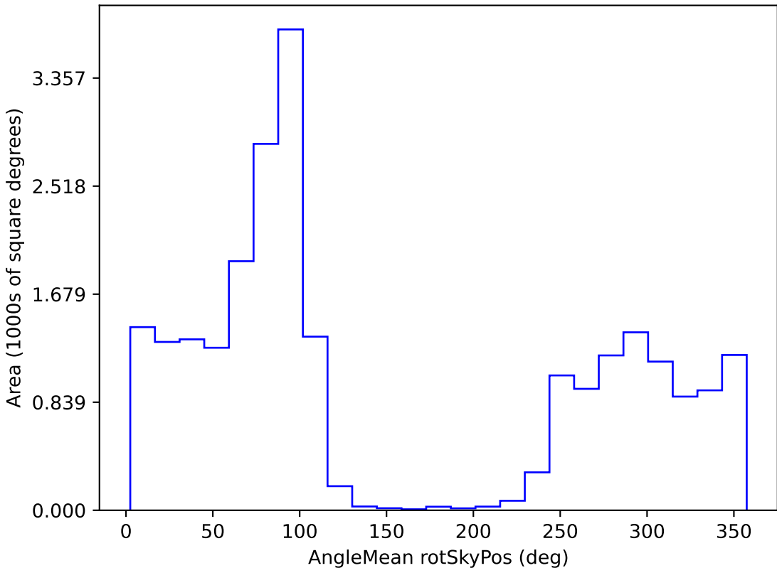
baseline_v3.5_10yrs All sky y band: AngleMean rotSkyPos
