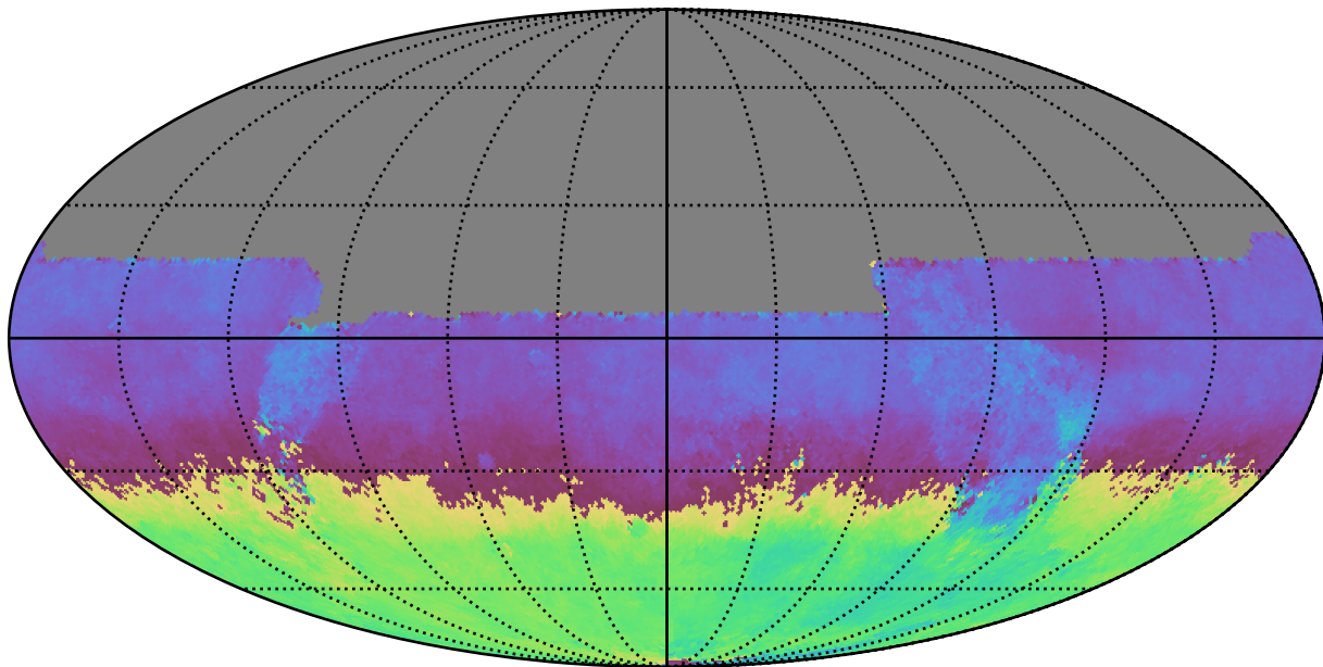
baseline_v3.5_10yrs All sky u band: AngleMean rotSkyPos
