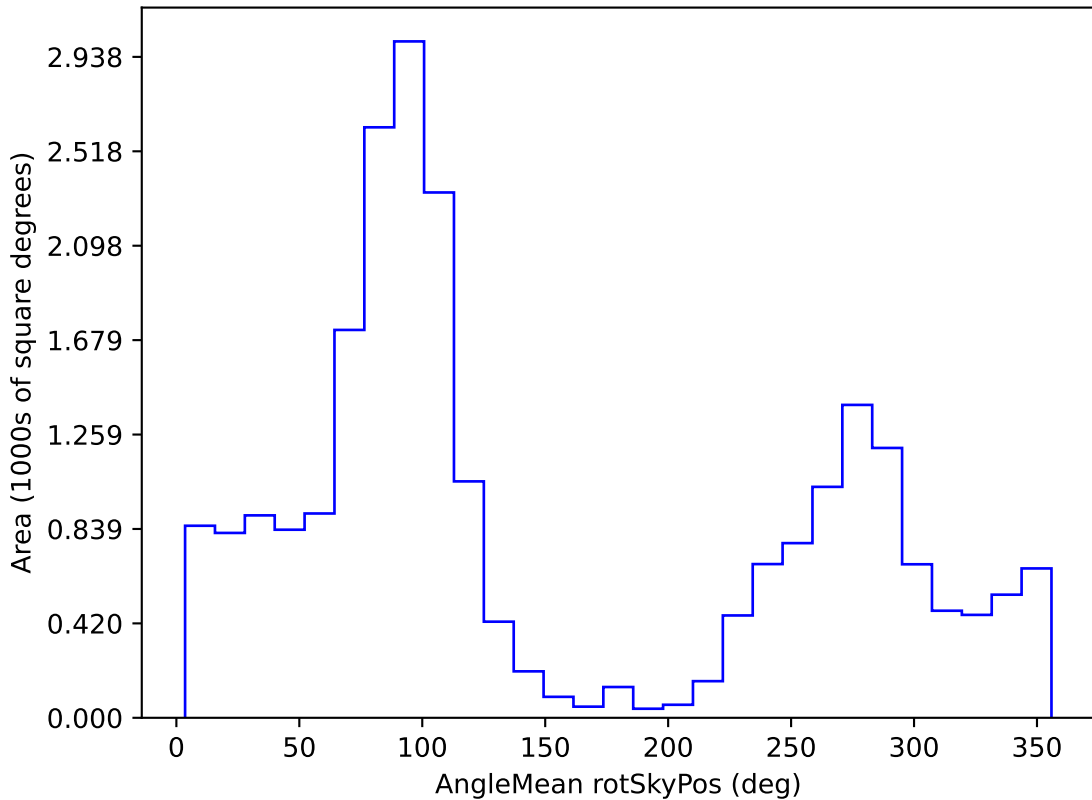
baseline_v3.5_10yrs All sky u band: AngleMean rotSkyPos
