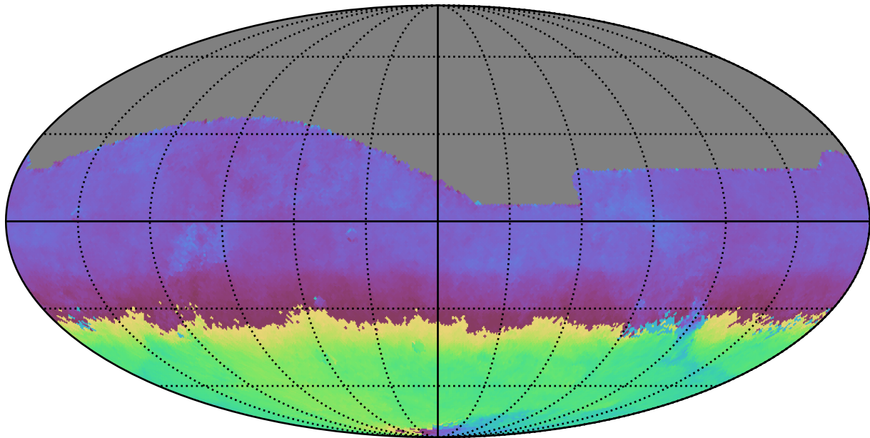
baseline_v3.5_10yrs All sky r band: AngleMean rotSkyPos
