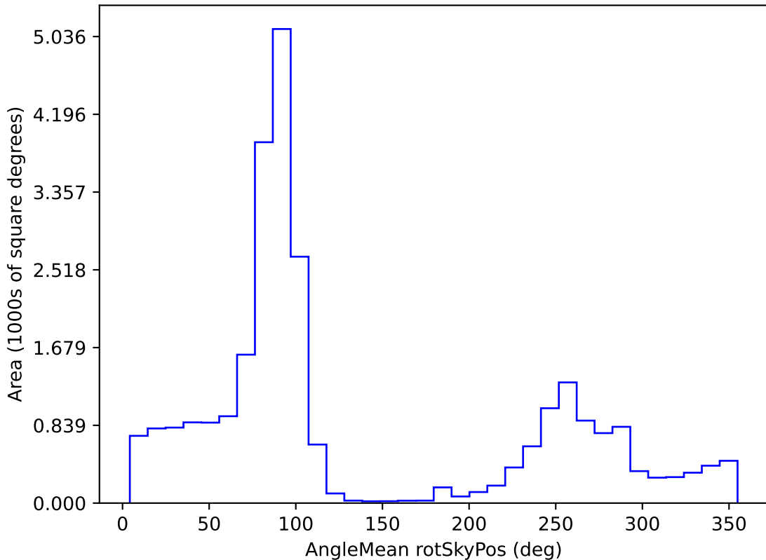
baseline_v3.5_10yrs All sky r band: AngleMean rotSkyPos
