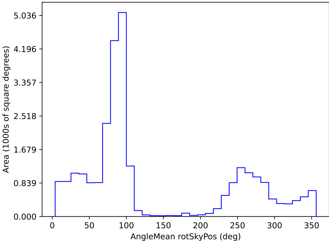
baseline_v3.5_10yrs All sky i band: AngleMean rotSkyPos
