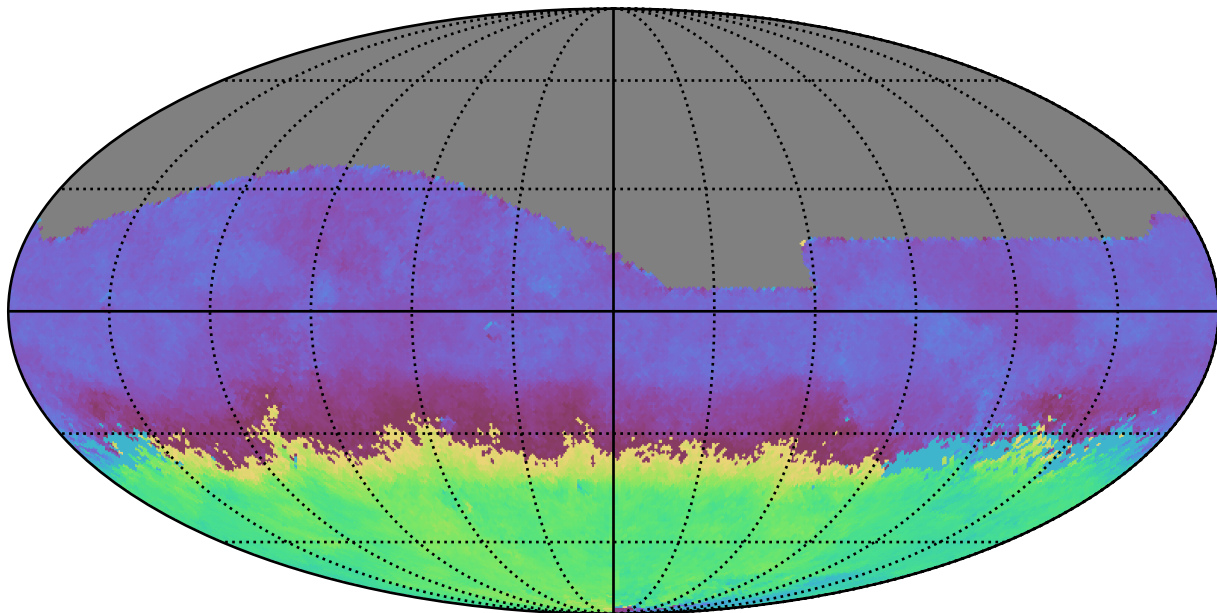
baseline_v3.5_10yrs All sky g band: AngleMean rotSkyPos
