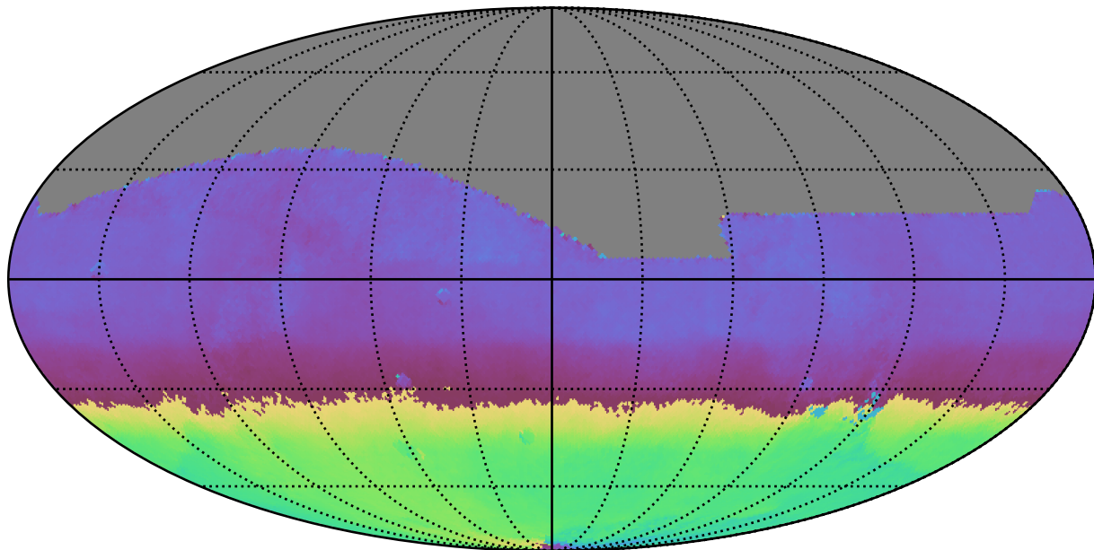
baseline_v3.5_10yrs All sky all bands: AngleMean rotSkyPos
