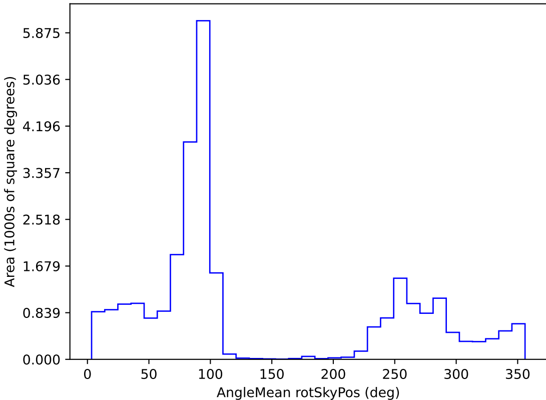
baseline_v3.5_10yrs All sky all bands: AngleMean rotSkyPos
