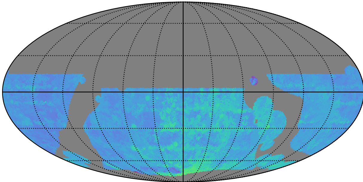
baseline_v3.5_10yrs WFD z band: 80thPercentile Season Length
