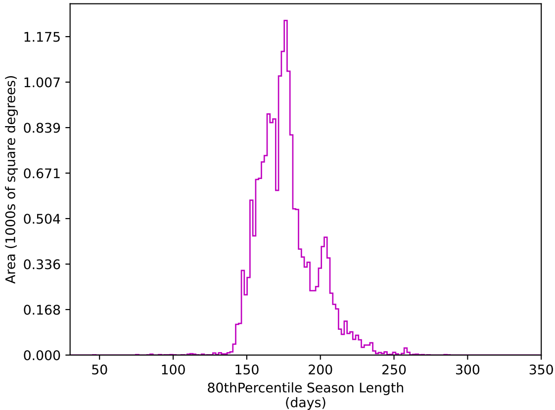
baseline_v3.5_10yrs WFD z band: 80thPercentile Season Length
