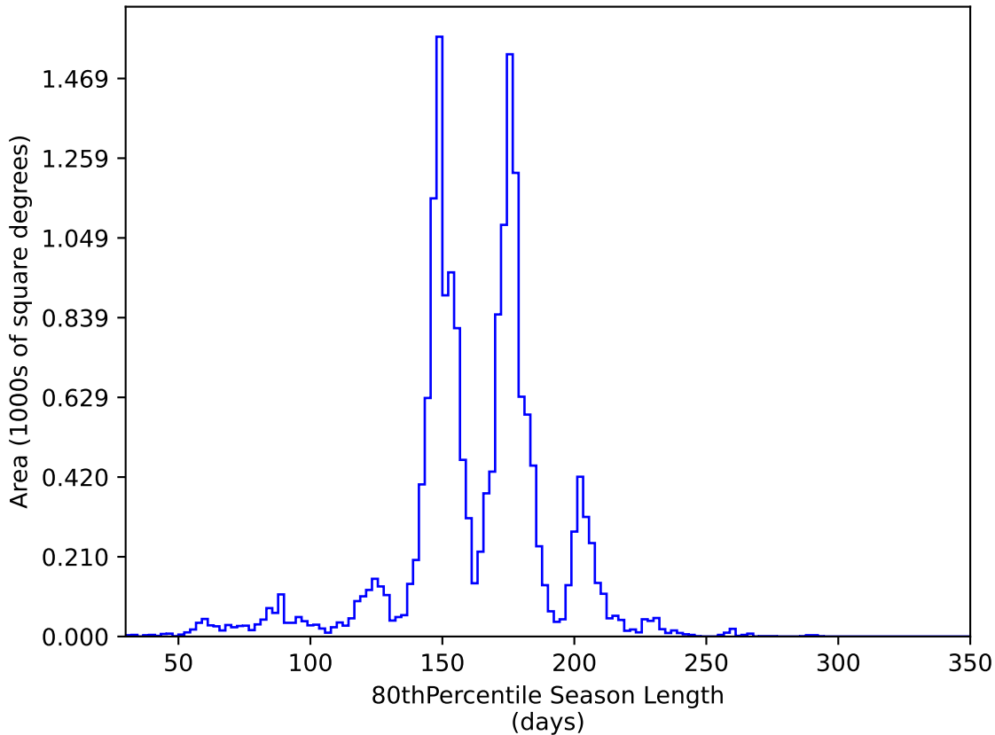
baseline_v3.5_10yrs WFD y band: 80thPercentile Season Length
