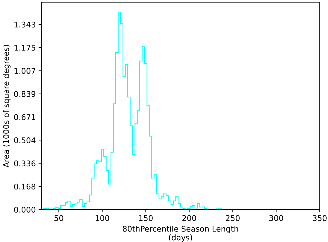
baseline_v3.5_10yrs WFD u band: 80thPercentile Season Length
