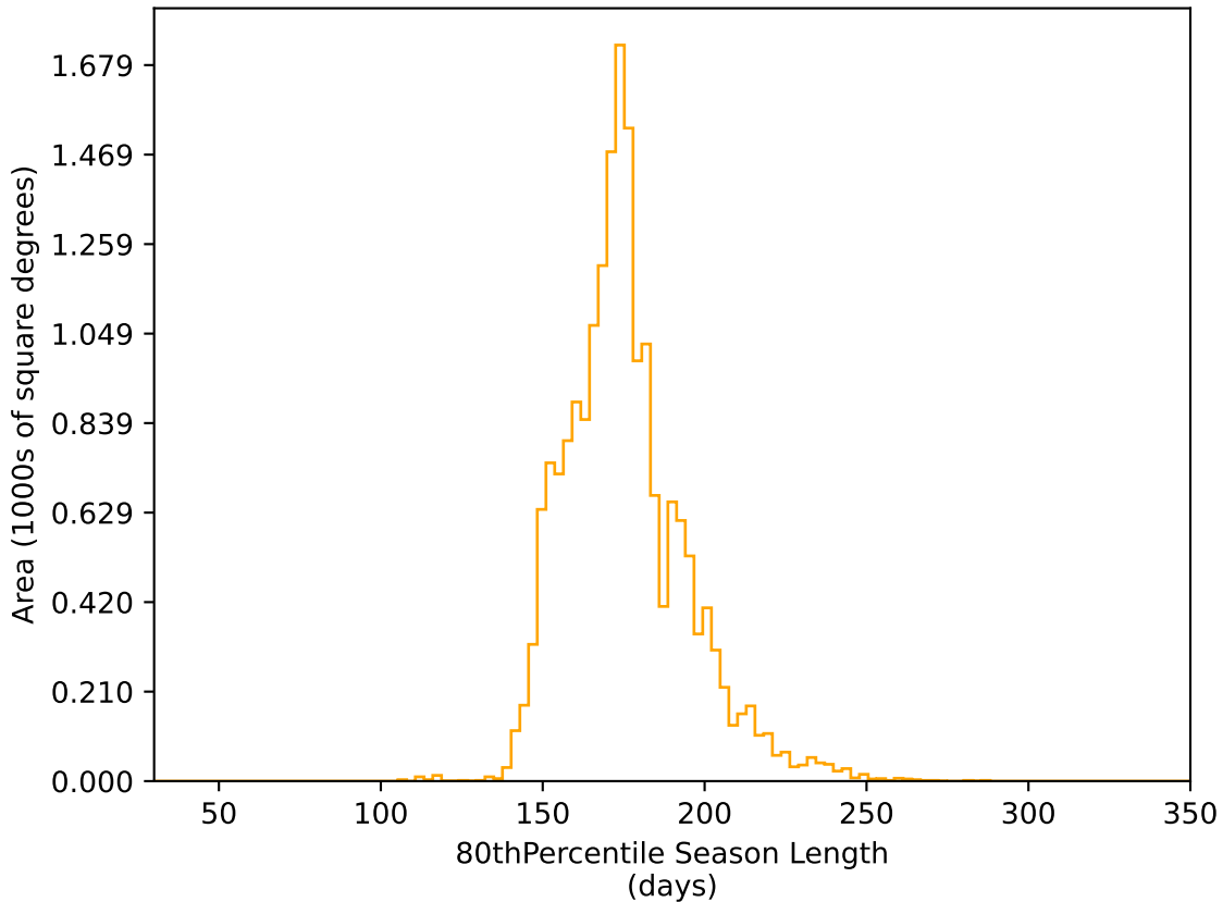
baseline_v3.5_10yrs WFD r band: 80thPercentile Season Length
